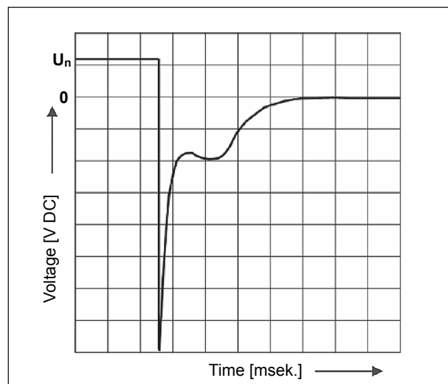
Fig. 9. DC coil voltage during switching off
