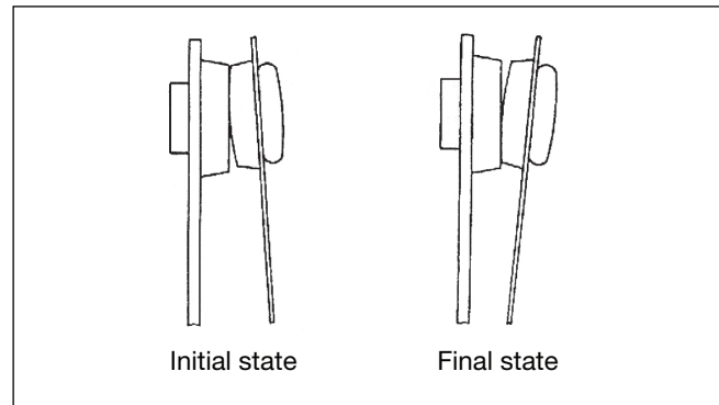
Fig. 13. Contact movement
