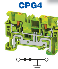
2 Connection Ground Terminal 2 Jumper Channels
